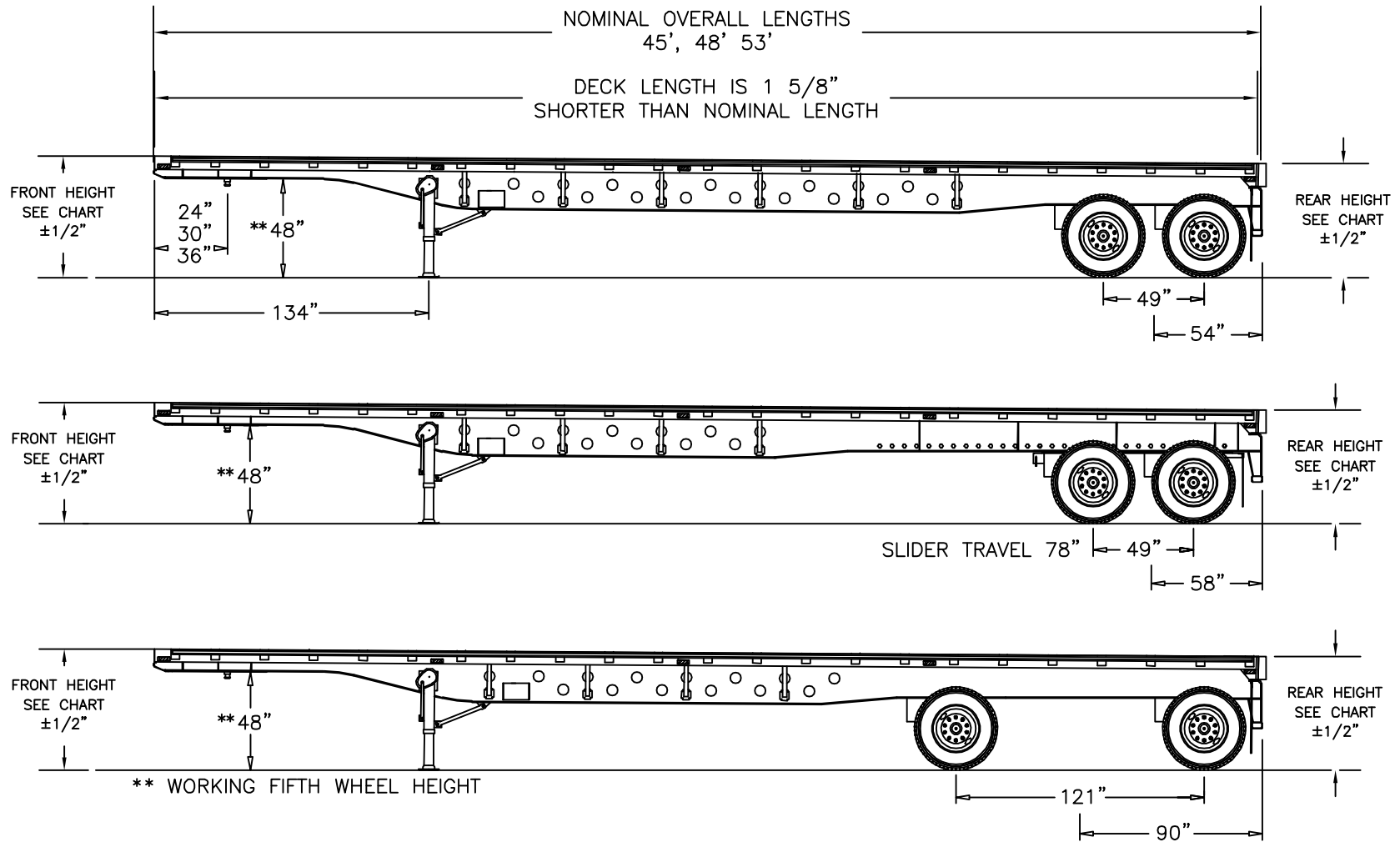
REAR HEIGHT VARIES WITH TIRE DIAMETER AND SUSPENSION SETTING
